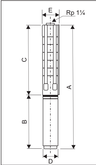
E - Max. diameter of the pump, including the cable guard and the motor
